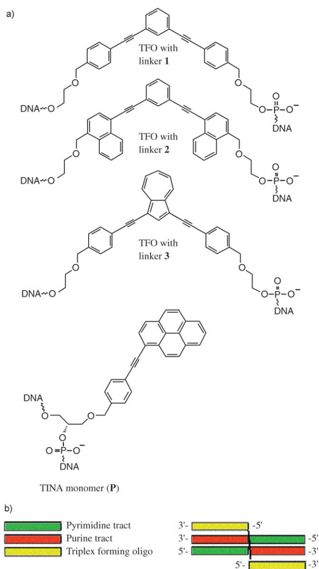
Scheme 1. a) Structures of the monomer of twisted intercalating nucleic acids ( P , TINA) and linkers for alternate strand TFOs ( 1–3 ). b) Representation of the 5'-5' alternate-strand triplex concept.
